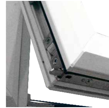
High security multipoint shootbolt lock. When activated, shootbolts engage firmly into keeps fitted to the window frame to add extra security.
